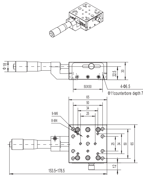
PSM25A-65C ▼
