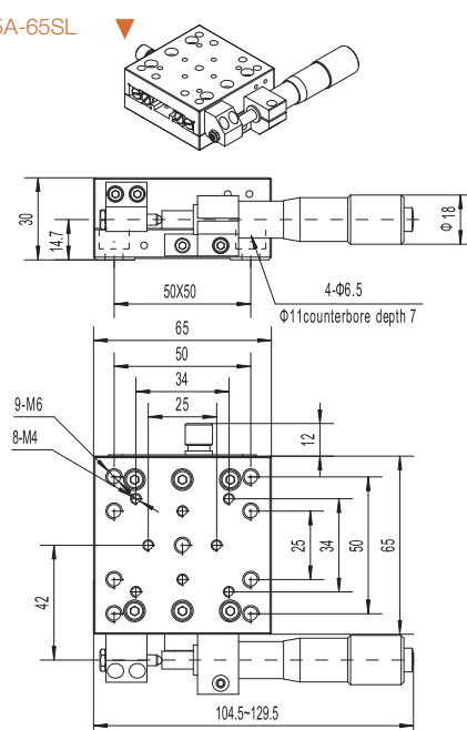
PSM25A-65SL ▼
